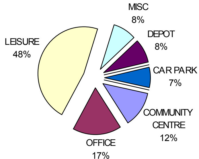
Buildings CO 2 Emissions Breakdown
